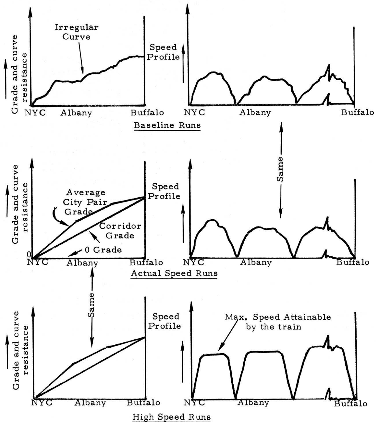
Figure 8.10 Velocity Profiles Under Various Track Conditions
