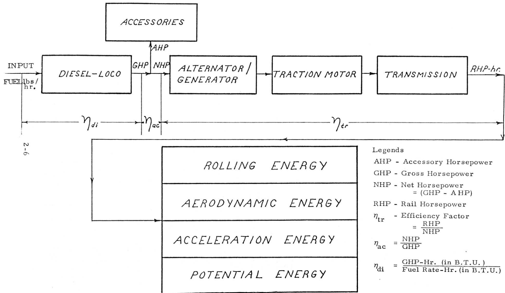
FIGURE 2.20 COMPONENTS OF ENERGY (ACCELERATION OR CRUISING)
